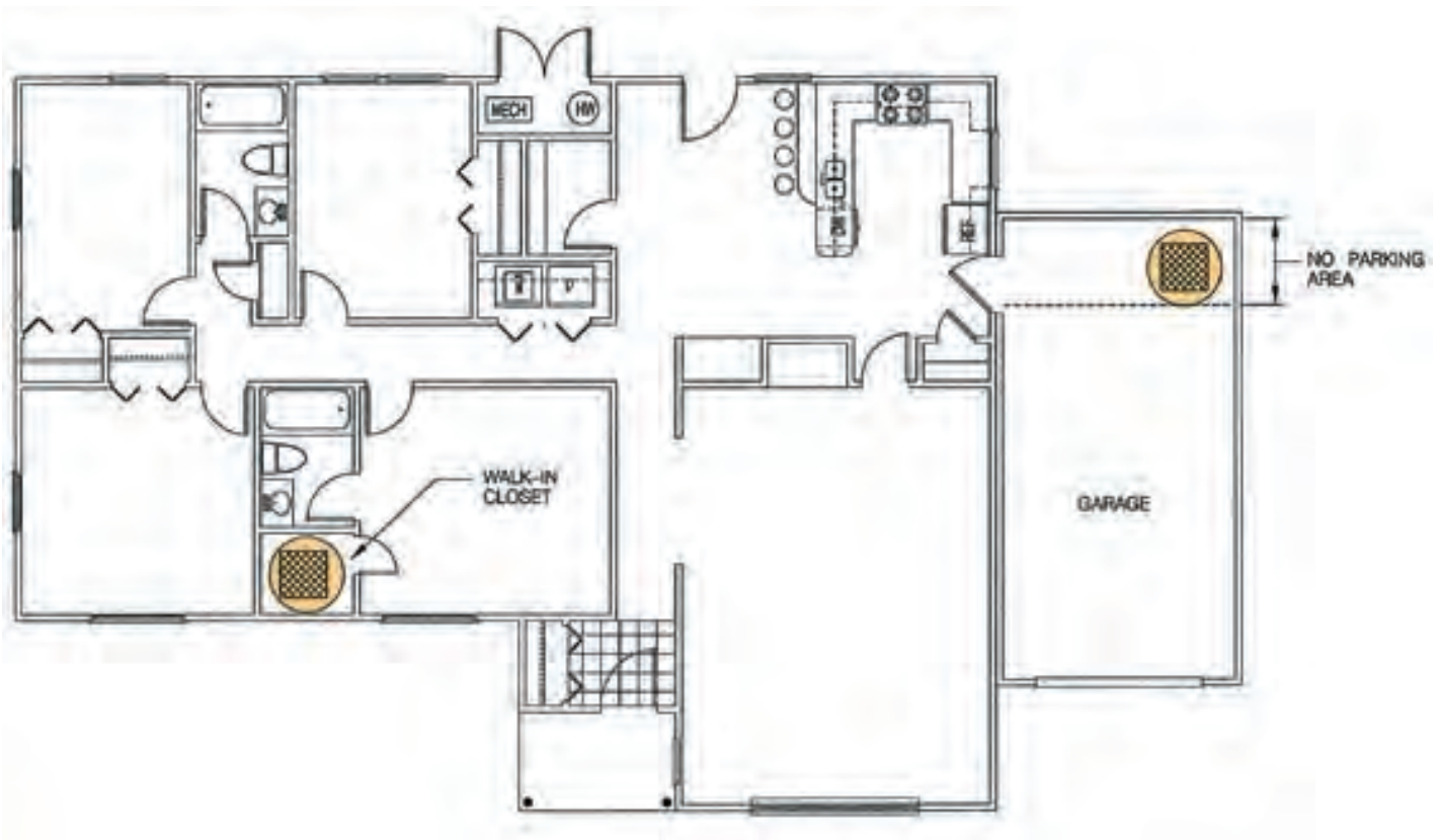
Figure II.7 Floor plan 3: house on slab-on-grade foundation
