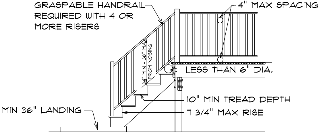
STAIR DETAIL
