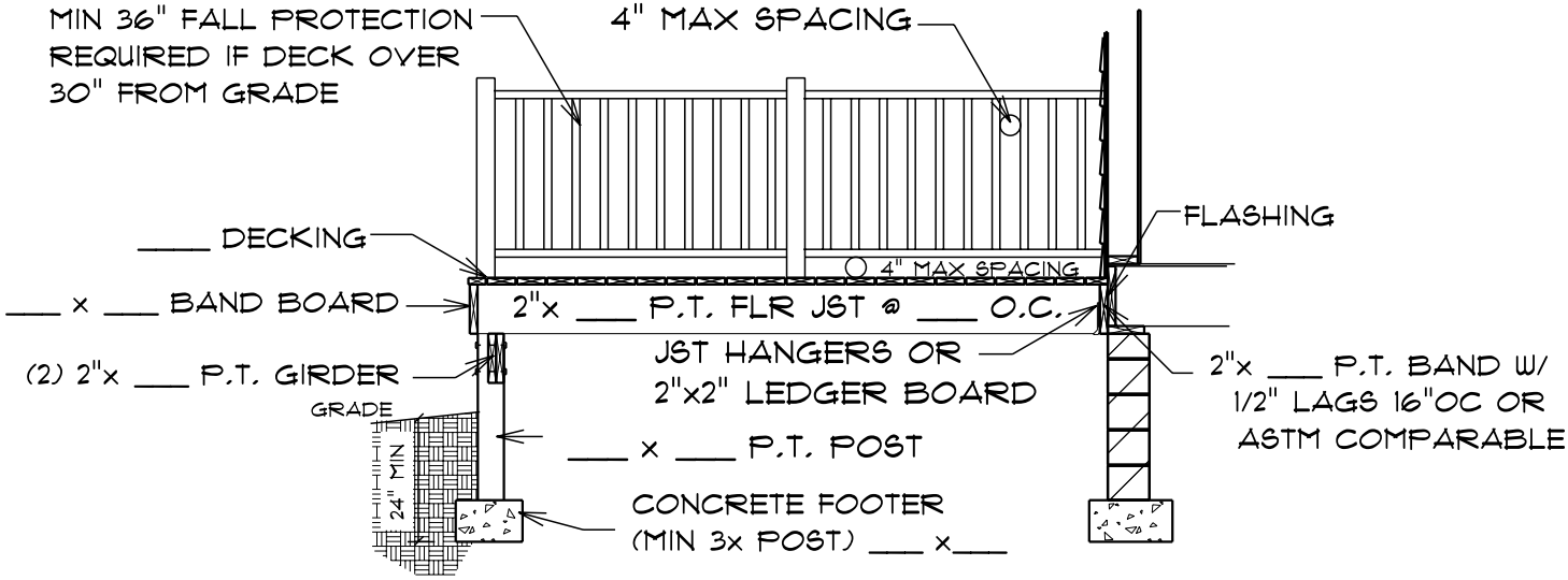
DECK SECTION
