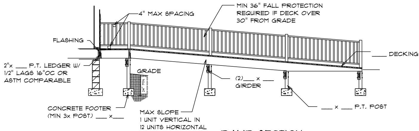
RAMP SECTION
