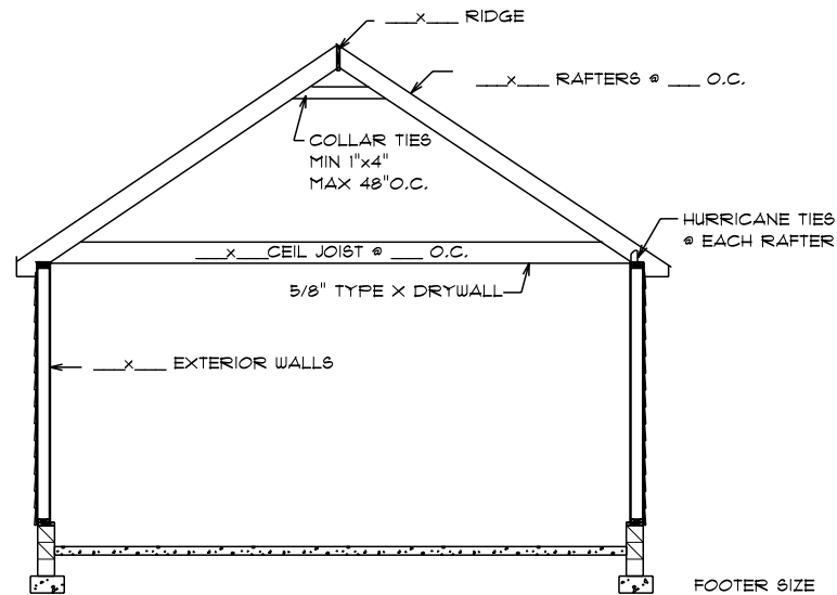
GARAGE SECTION
