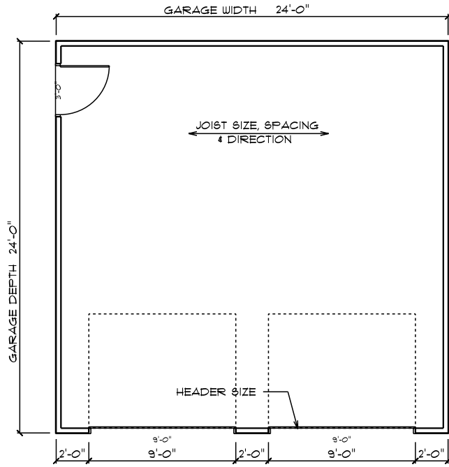
FLOOR PLAN
