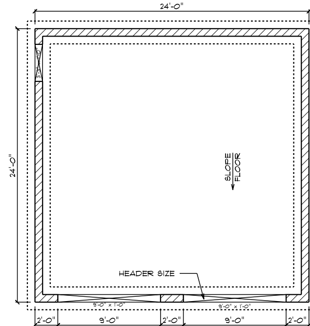
FOUNDATION
