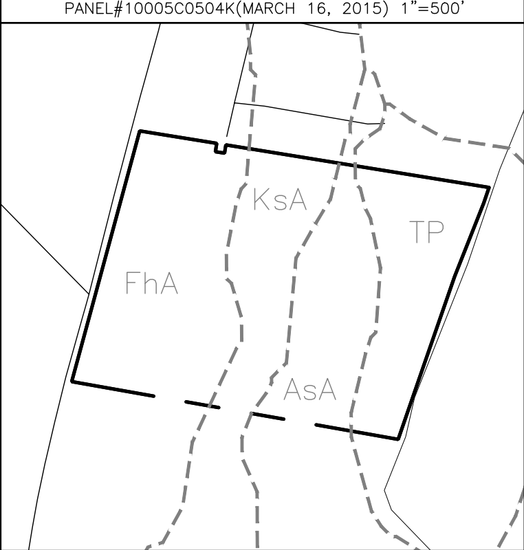
SOILS MAP 1"= 500'
